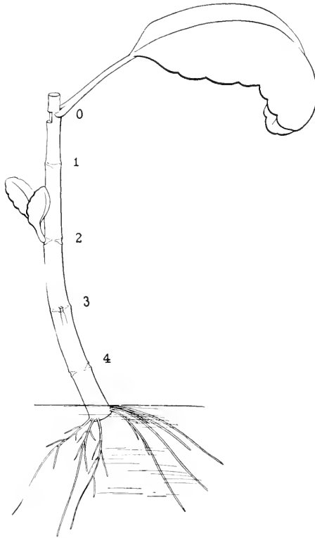
FIG. 72.—Young stem with one apical leaf. Bud opposite the leaf (in node 0) is cut out. Shoot formation in the first node below the leaf is suppressed, but a shoot is formed in the second node below and opposite the leaf.
